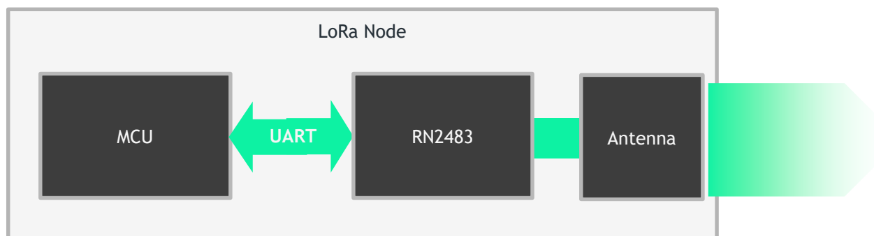
Diagram 2: A typical LoRa Node setup
